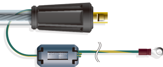
Plate type VXH-W102 Standard Accessory
